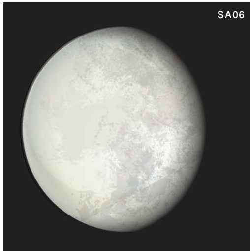
waning gibbous
