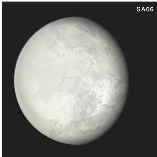
waning gibbous
