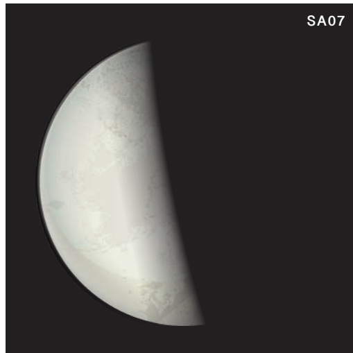
third quarter
