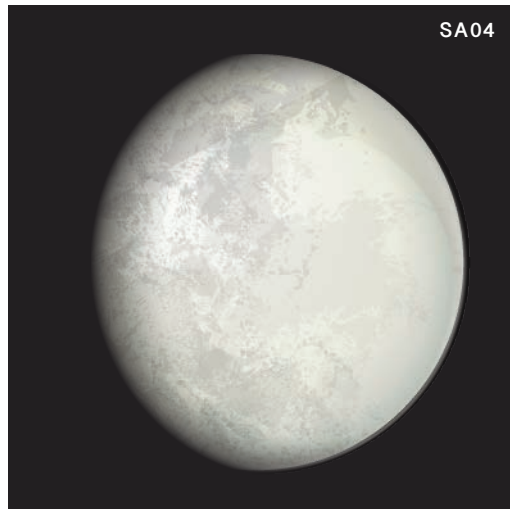
waxing gibbous
